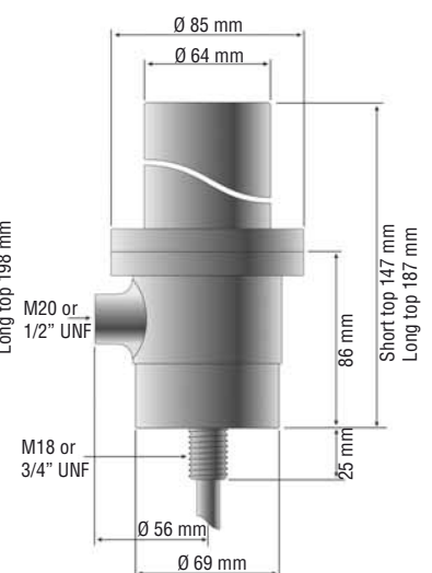
Side mounted cable gland
